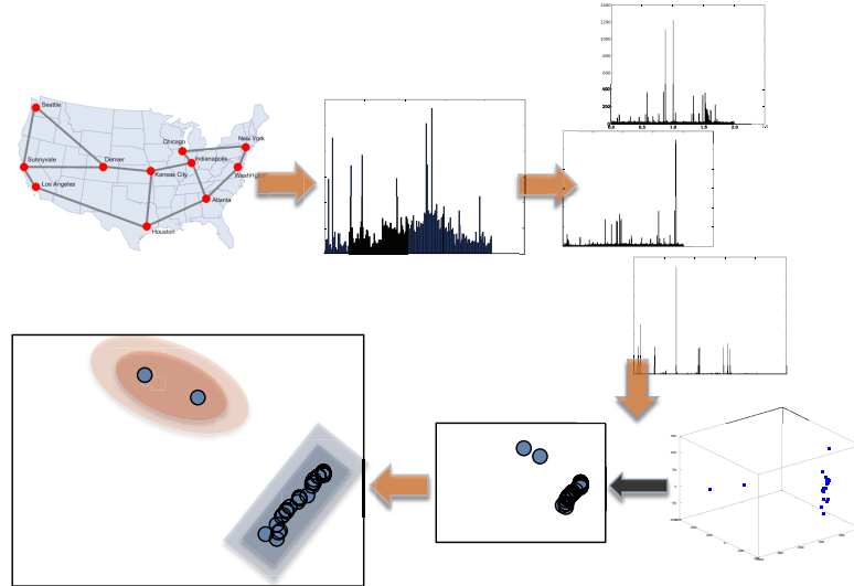
Fig. 1. Depiction of the pipeline. Each orange arrow represents one phase of the four-step process. Step 1, the sensor process, converts high dimensional heterogeneous data into a structured data stream representation. Step 2, the attention process, determines an attention trigger, extracts high-dimensional event data, and applies an alignment algorithm to align events in time. The result is a high-dimensional matrix. Step 3, the pattern process, employs pattern-discovery algorithms (gray arrow) to convert the high dimensional input into a lower-dimensional representation. Step 4, the interpretation process, characterizes the domains in the lower-dimensional representation space and makes it possible to distinguish normal system operations from system vulnerability or failure.
