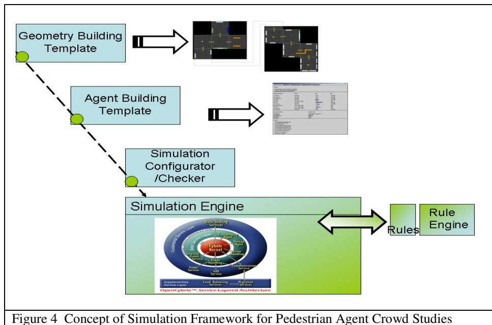
Figure 4 Concept of Simulation Framework for Pedestrian Agent Crowd Studies
