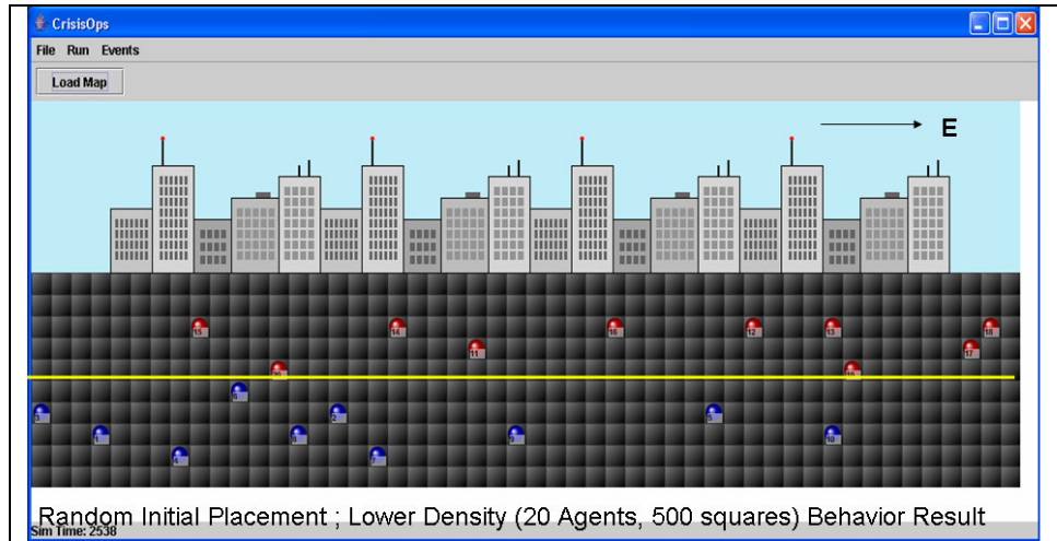
Figure 1: Spontaneous Lane Formation. Westward (red dots) moving pedestrians and eastward (blue dots) moving pedestrians separate into lanes. Not only is there lane formation, the entire westward flow has a sharp boundary from the eastward moving pedestrian flow.
