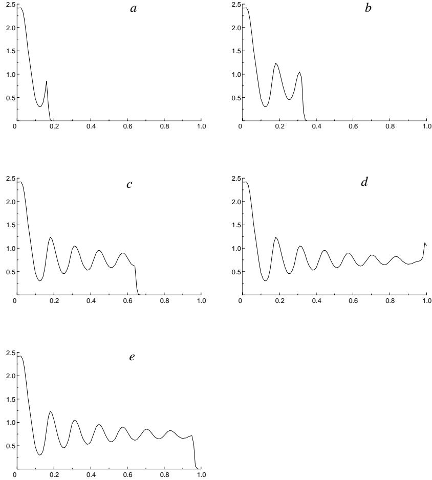
Figure 4. Dynamics of fungal colony development resulting in concentric rings formation ( x -axis is relative radius, y -axis is relative mycelium density). Parameters of the model: \nu = 1.2 ; \rho^0 = 0.03 ; \xi^0 = 0.1 ; \lambda = 7 ; \varepsilon = 0.40 ; s^0 = 10 ; D_s = 5.0 \cdot 10^{-5} ; \gamma = 1 ; D_m = 0.001 ; \alpha = 0.5 ; \mu^0 = 0.1 ; \tau^0 = 0.50 ; \eta = 0.90 . Time: a - \tau = 4.2 ; b - \tau = 8.3 ; c - \tau = 16.7 ; d - \tau = 25.0 ; e - \tau = 33.3 .
