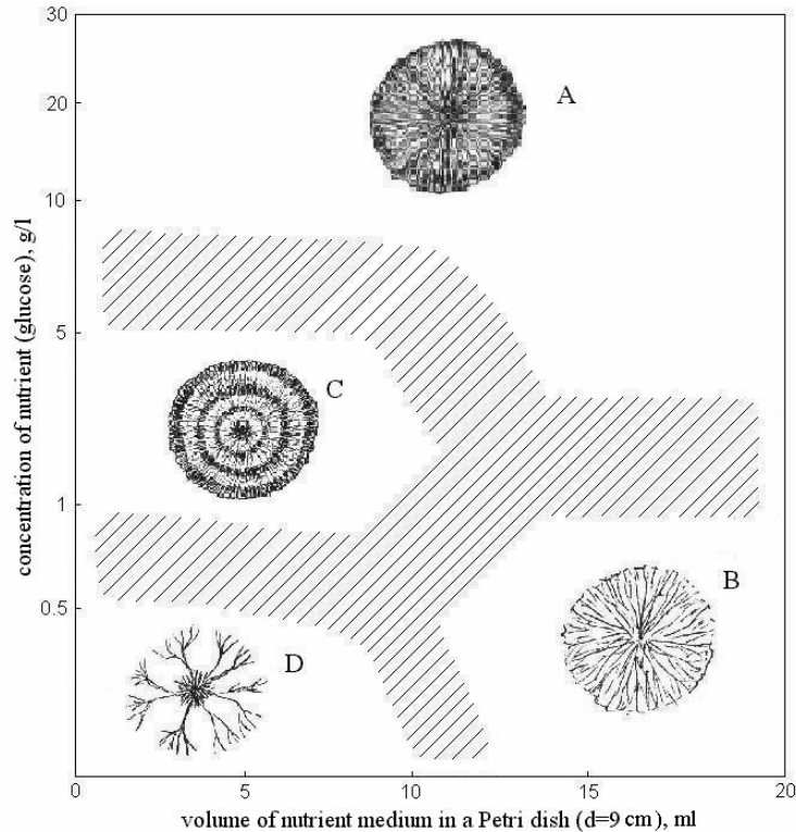
Figure 2. Morphological diagram of fungal colony patterns: A – “dense lawn”, B – “sparse lawn”, C – concentric rings, D – fractal-like structures.
