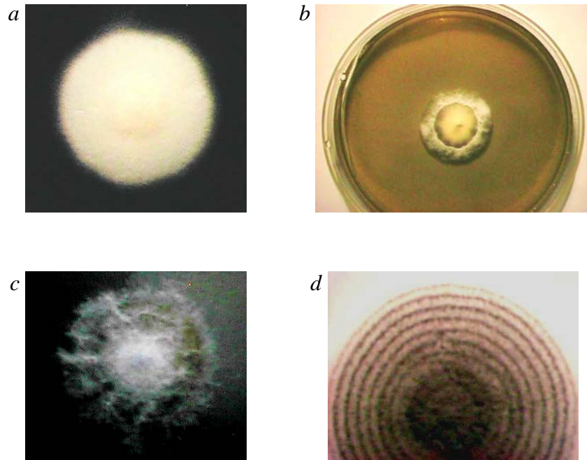
Figure 1. Different growth patterns which can develop in colonies of mycelial fungi: a – “dense lawn”, b – “sparse lawn”, c – fractal-like structures, d – concentric rings.
